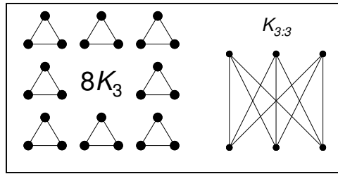
Fig. 5.7. The graphs 8K_3 and K_{3,3} .
