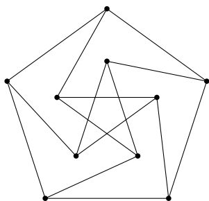
Figure 1: Peterson graph
