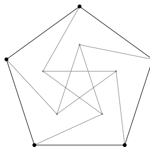
Figure 2: Induced Subgraph of Peterson graph
